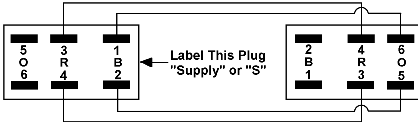
4 Wire Cable (Far Block Control Cable)
