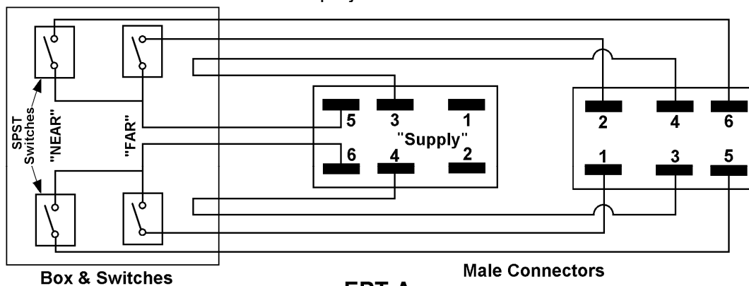
EPT-A "Black Box" Module Control
